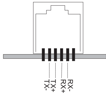
Pin assignment of DA,DX & M -series (RJ-11 Viewed via end-cap )
